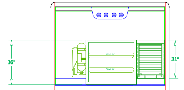
FRONT VIEW CROSS-SECTION
