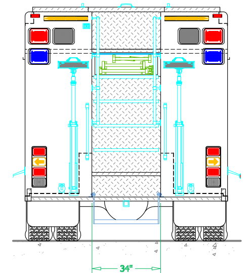
REAR VIEW CROSS-SECTION
