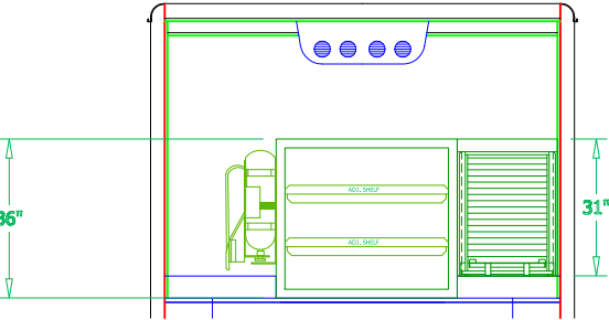
FRONT VIEW CROSS-SECTION
