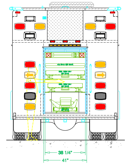
CHASSIS INTERIOR REAR CROSS-SECTION
