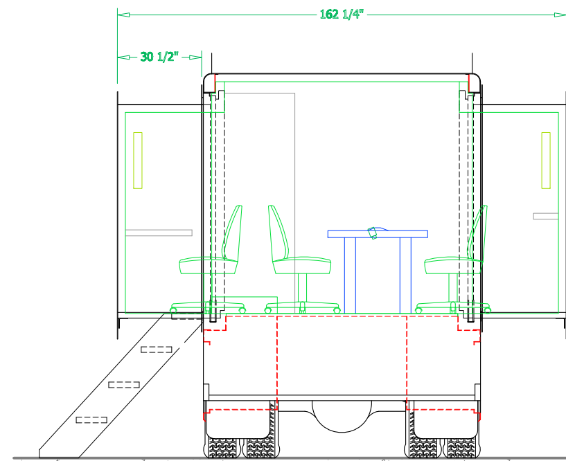
REAR VIEW CROSS-SECTION
