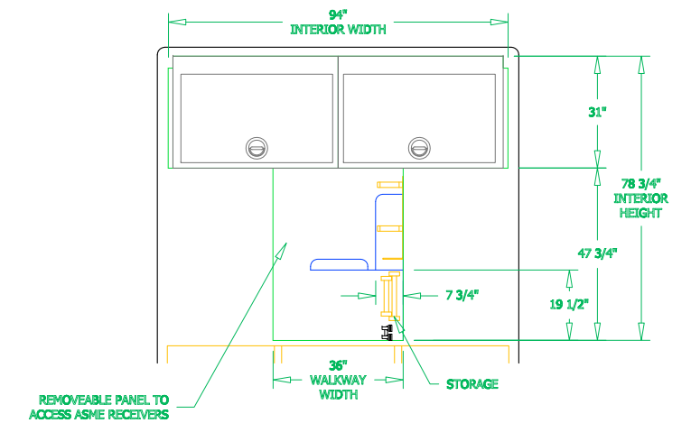
REAR VIEW CROSS-SECTION
