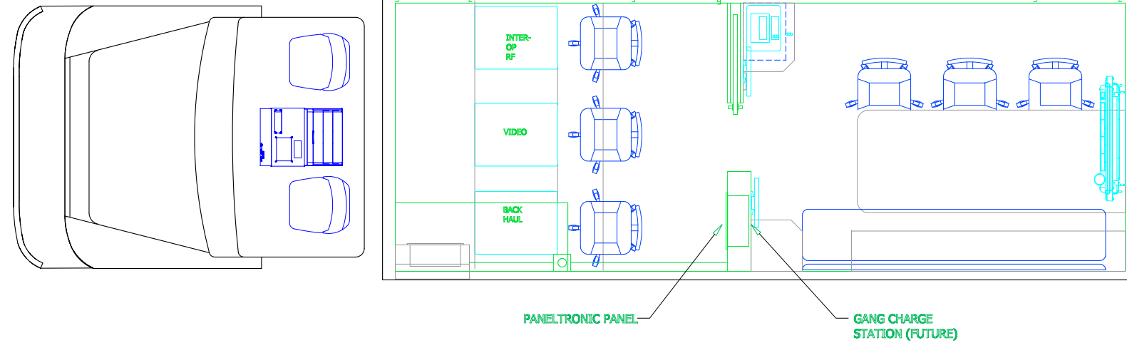
PLAN VIEW CROSS-SECTION
