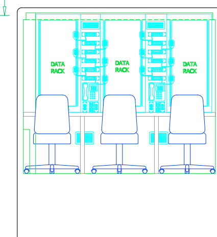
STREETSIDE INTERIOR CROSS-SECTION
