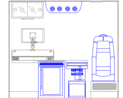
CHASSIS FRONT VIEW CROSS-SECTION
