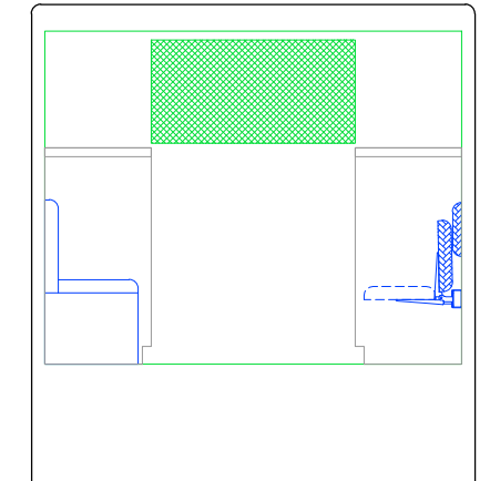
FRONT VIEW CROSS-SECTION
