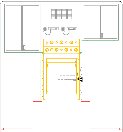
FRONT VIEW CROSS-SECTION
