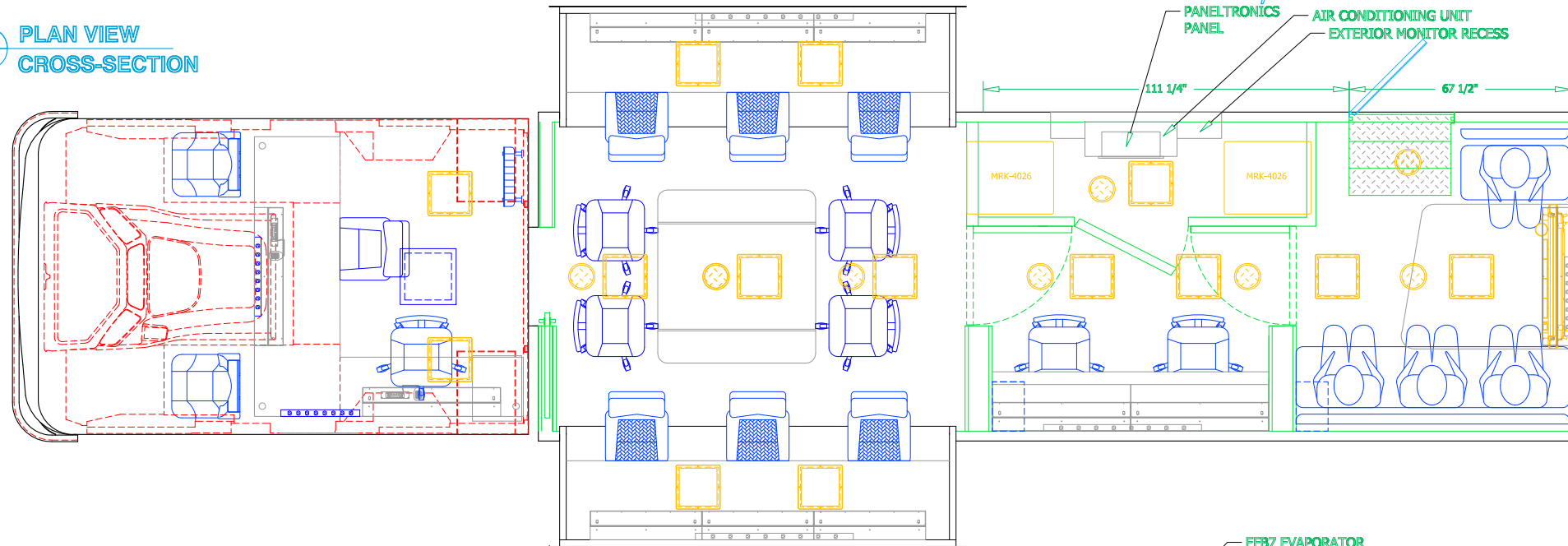
CURBSIDE INTERIOR CROSS-SECTION
