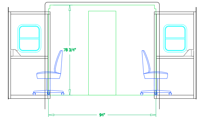
REAR VIEW CROSS-SECTION
