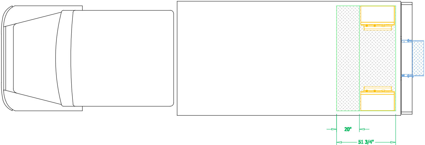
PLAN VIEW CROSS-SECTION
