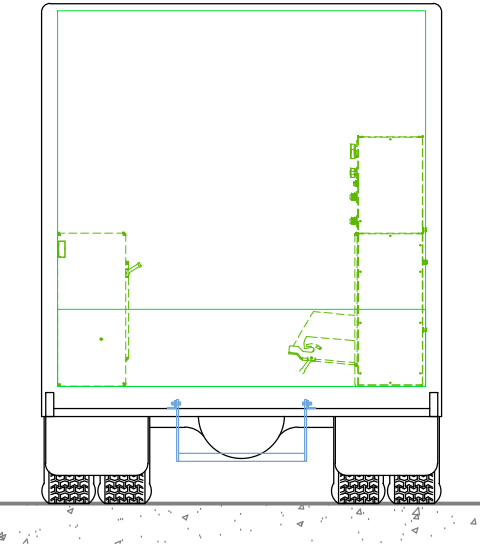
REAR VIEW CROSS-SECTION
