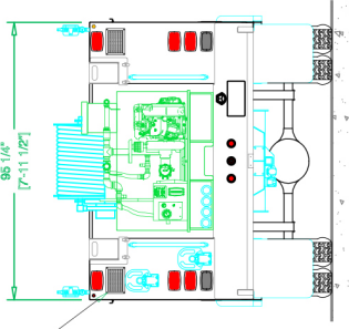
(2) WHELEN PIONEER PCPSM/C FLUSH MOUNT SPOT/FLOODLIGHTS (1 EACH SIDE)
