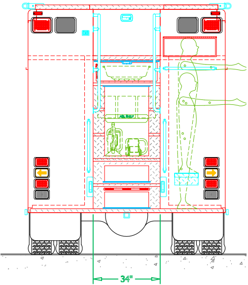
TOOLBOARD LAYOUT - S4
