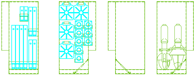
TOOLBOARD LAYOUT - S4
