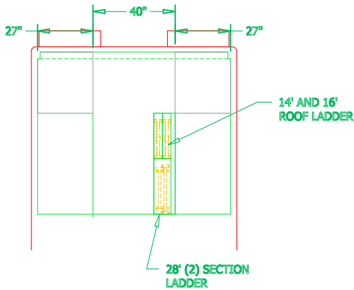
REAR VIEW CROSS-SECTION
