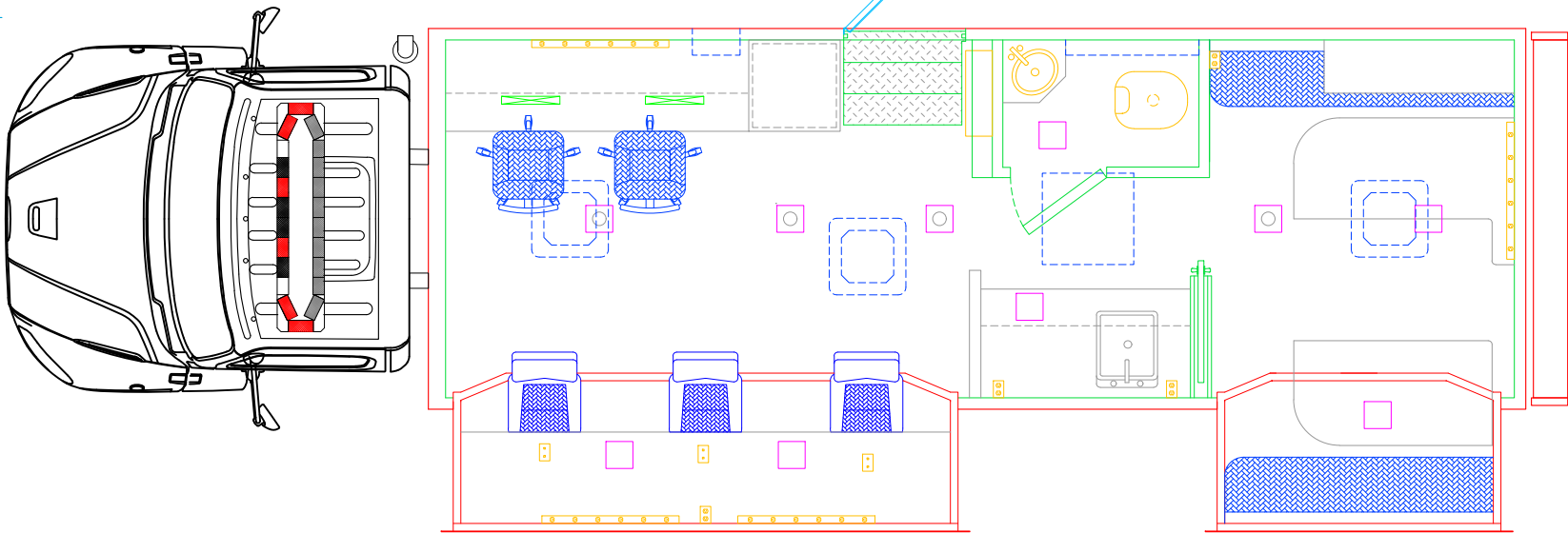
PLAN VIEW
