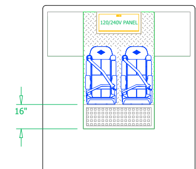
WALK-IN CROSS-SECTION
