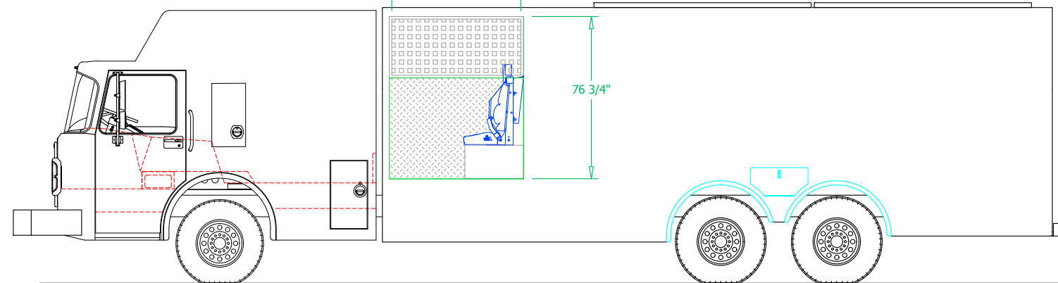
CURBSIDE INTERIOR CROSS-SECTION
