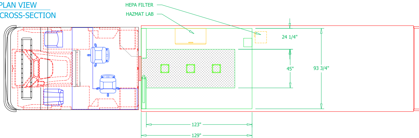
CURBSIDE INTERIOR CROSS-SECTION
