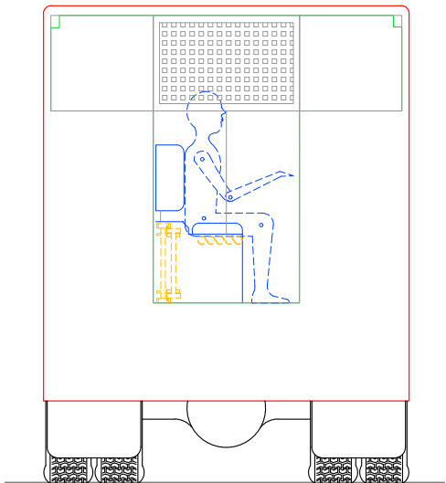
REAR VIEW CROSS-SECTION
