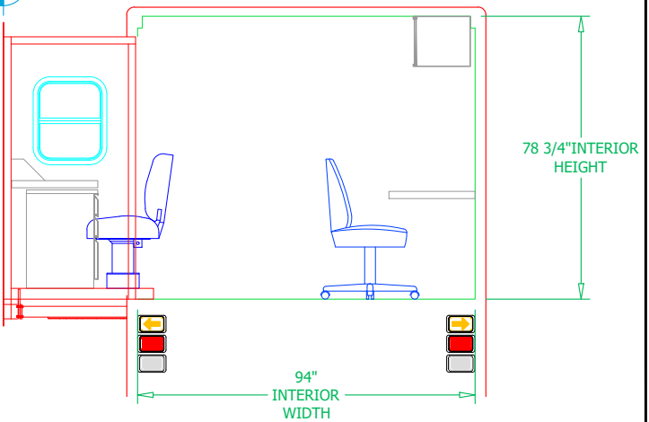
REAR VIEW
