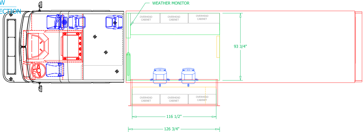
CURBSIDE INTERIOR CROSS-SECTION
