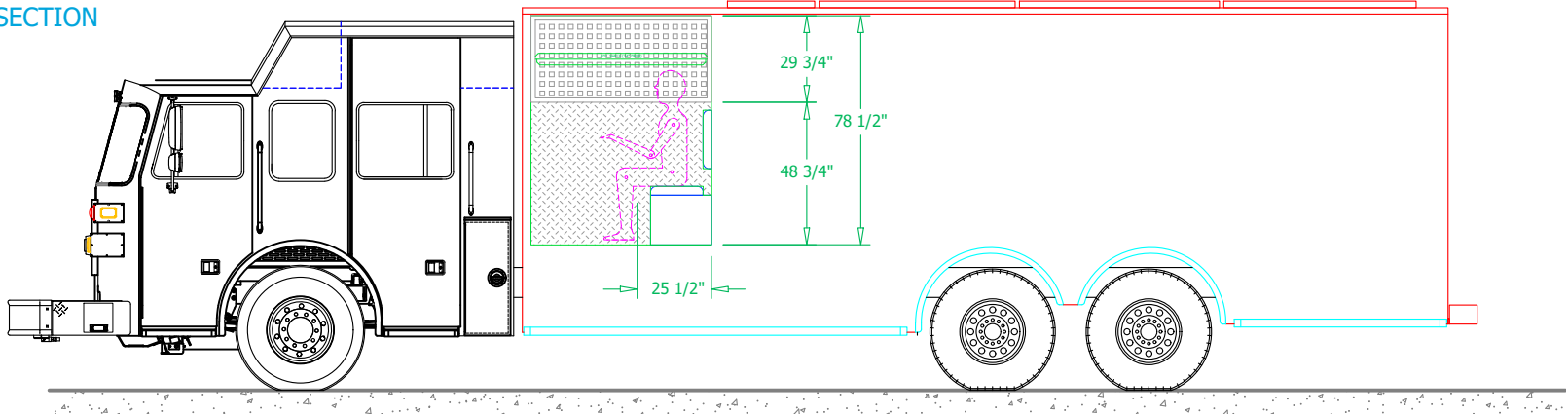
CURBSIDE INTERIOR CROSS-SECTION
