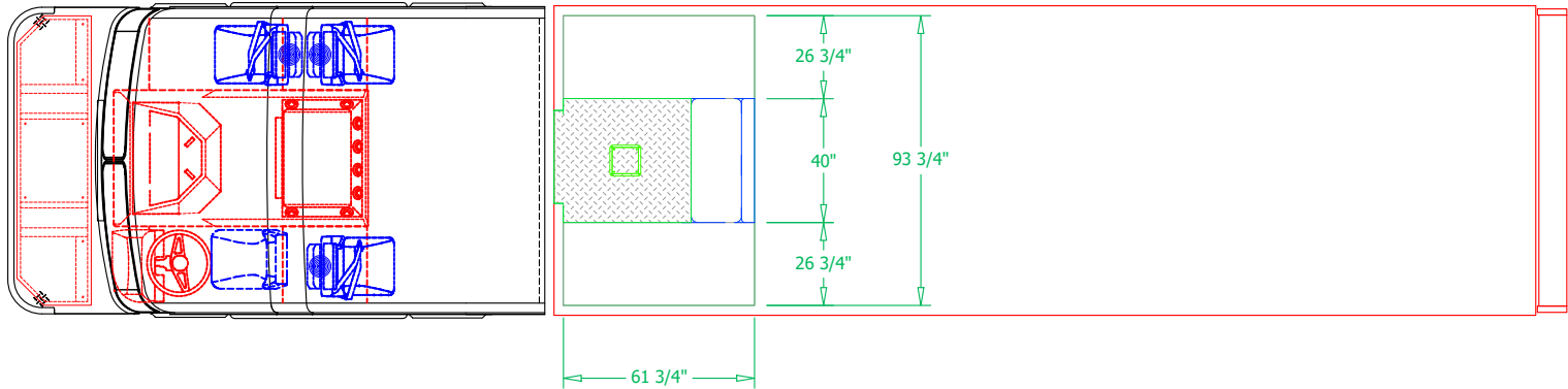
PLAN VIEW CROSS-SECTION
