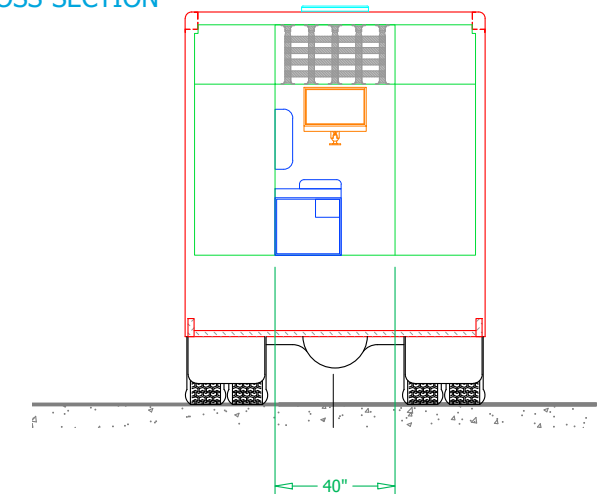
REAR VIEW BODY CROSS-SECTION
