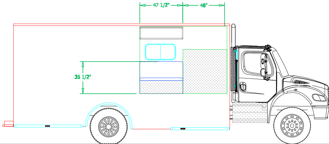
STREETSIDE INTERIOR CROSS-SECTION
